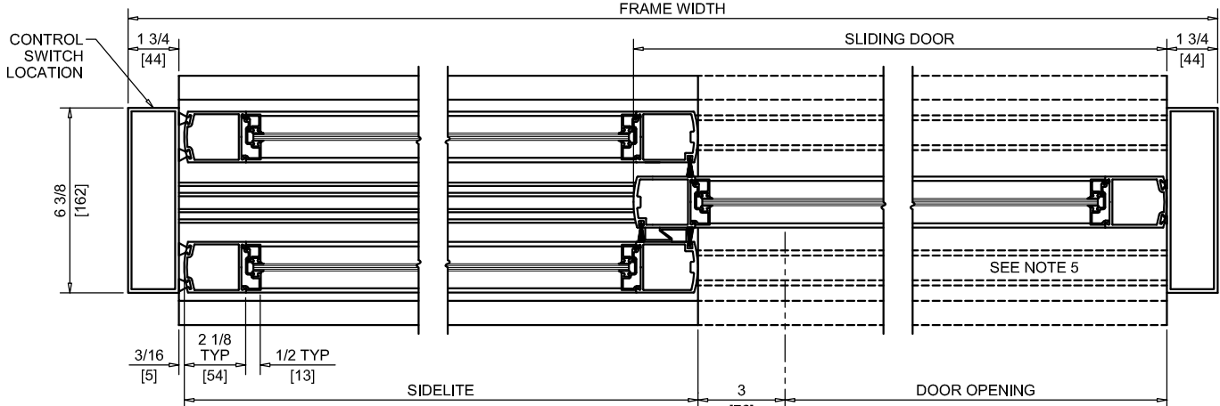
HORIZONTAL SECTION
