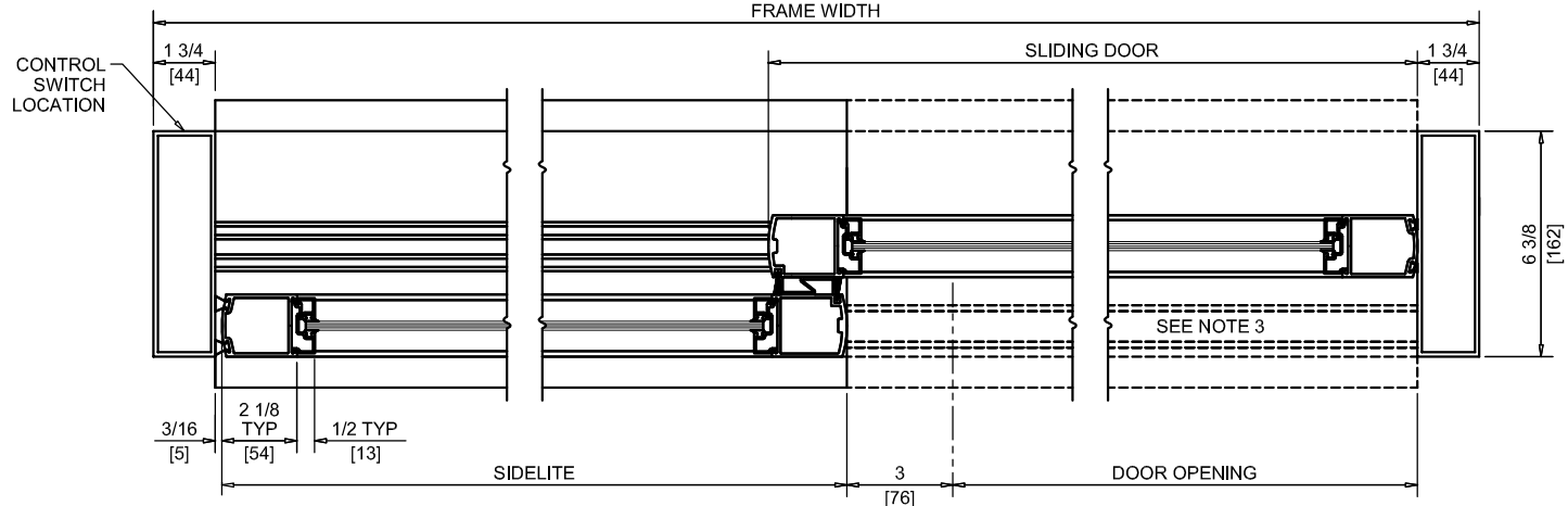
HORIZONTAL SECTION
