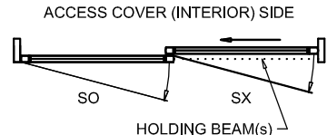
EXTERIOR ELEVATION/PLAN
