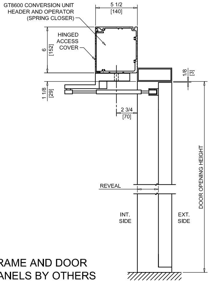
VERTICAL SECTION BUTT/OFFSET PIVOT OPTION
