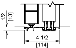
RECESSED TRACK (OPTIONAL)
