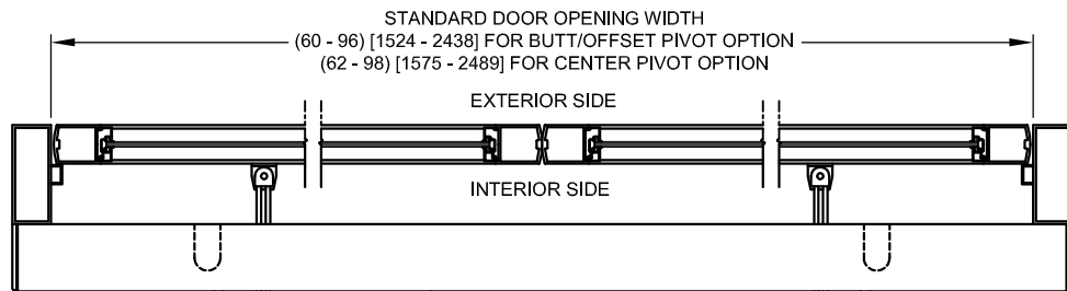
HORIZONTAL SECTION
