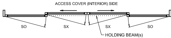
EXTERIOR ELEVATION/PLAN
